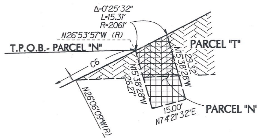
DETAIL "B" NO SCALE
